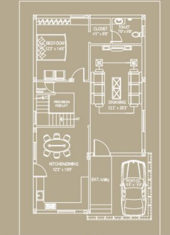
50' EAST ROAD GROUND FLOOR PLAN
