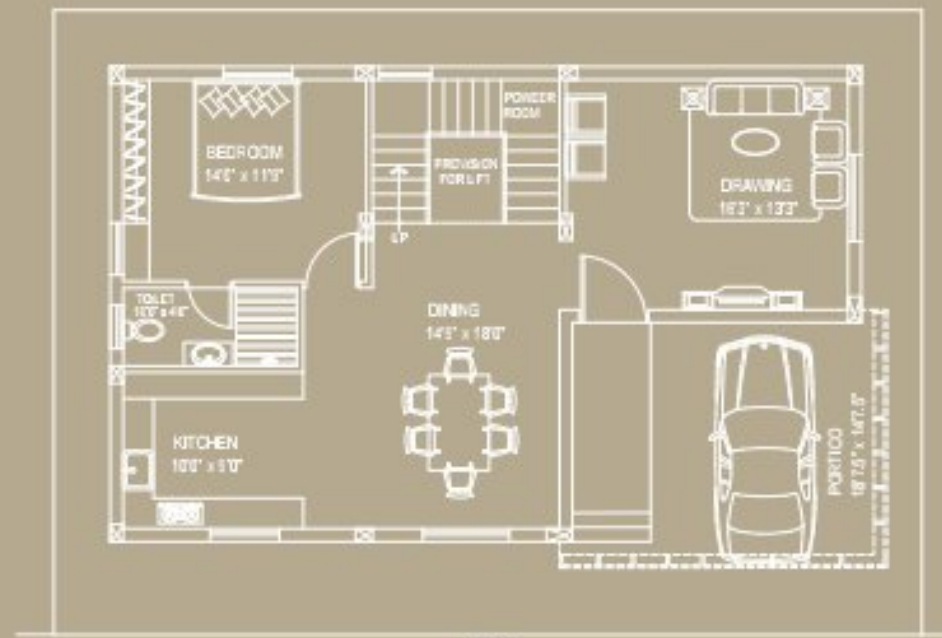
50'0" EAST ROAD GROUND FLOOR PLAN
