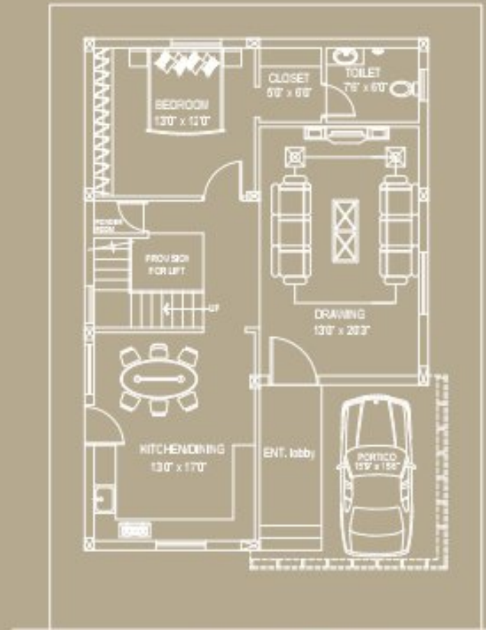
EAST ROAD GROUND FLOOR PLAN
